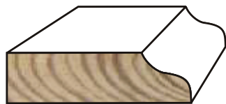
916 L 3/8" x 1-3/8" Length 17'
