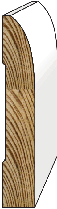
713 9/16" x 3-1/4"
