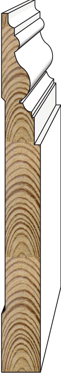
PM6 11/16" x 6-1/4"
