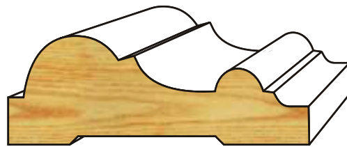
AM 214PP 13/16" x 2-1/4"
