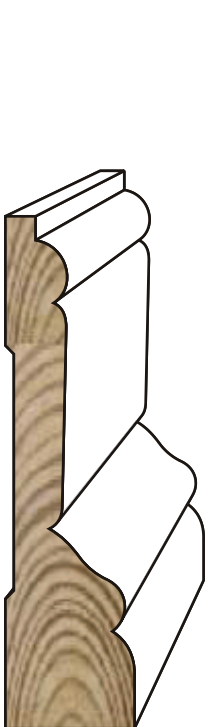
462 11/16" x 2-3/4"
