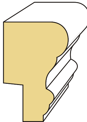
w/ 3/8" x 11/16" Rabbet LDF 850M 1-1/8" x 1-3/4" Wainscot Cap
