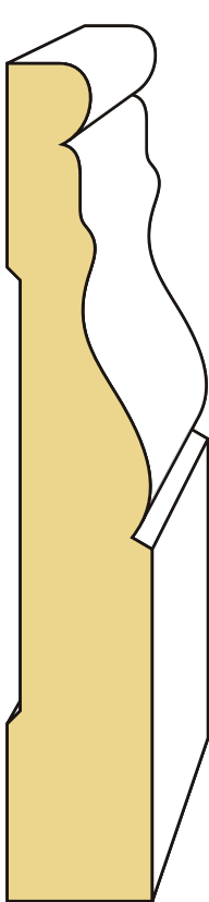
LDF 214 3/4" x 4"
