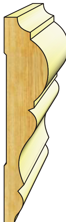
CH 312 3/4" x 3-1/2"
