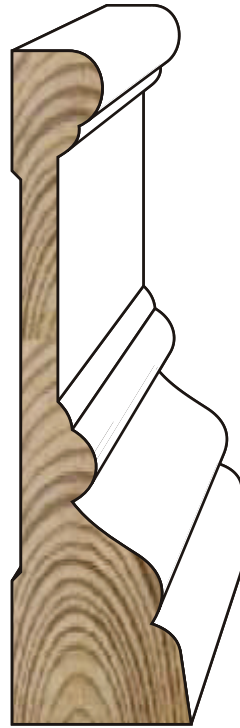
RB3 1" x 3-1/2"
