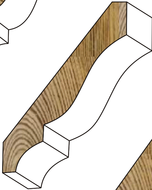
49 9/16" x 3-5/8"
