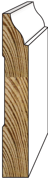
623 9/16" x 3-1/4"
