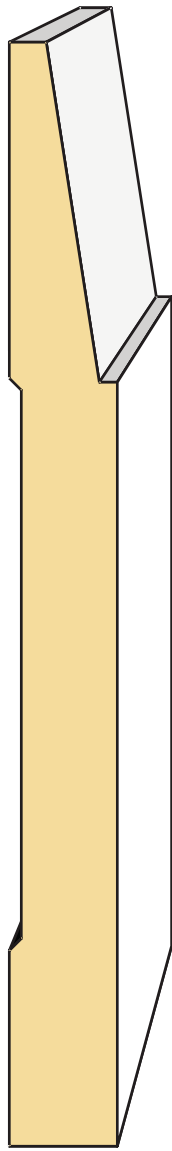
LDF BA534A 9/16" x 5-3/4"
