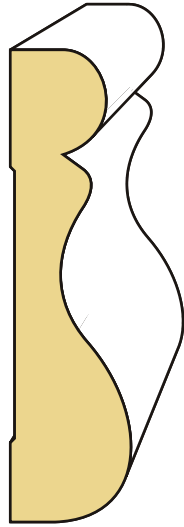
LDF 914 5/8" x 2-7/16" Base Cap
