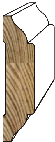
224 9/16" x 2-1/4"
