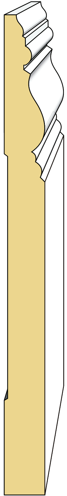
LDF BA914 3/4" x 9-1/4"
