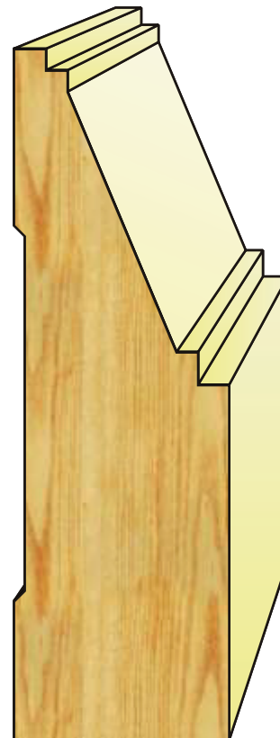
CA 35A 3/4" x 3-1/2"
