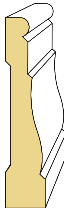
LDF 445 11/16" x 3-1/4"
