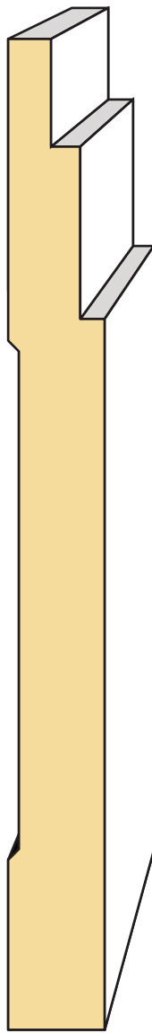
LDF BA534B 9/16" x 5-3/4"
