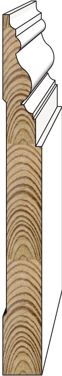
PM6 11/16" x 6-1/4"
