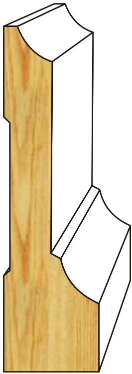
CA 358PP 1" x 3-5/8"
