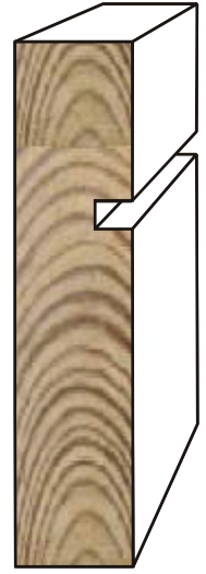
212N 11/16" x 2-1/2"
