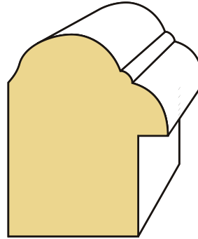
w/ 1/4" X 3/4" Rabbet LDF BB112 1-3/16" x 1-1/2" Back Band
