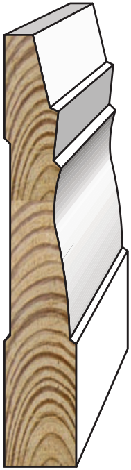
366 B 9/16" x 3-1/4"
