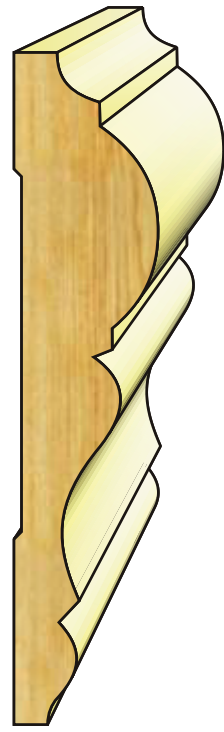
CH 312 3/4" x 3-1/2"
