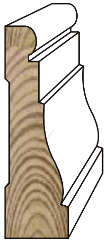
376L 11/16" x 2-1/4"
