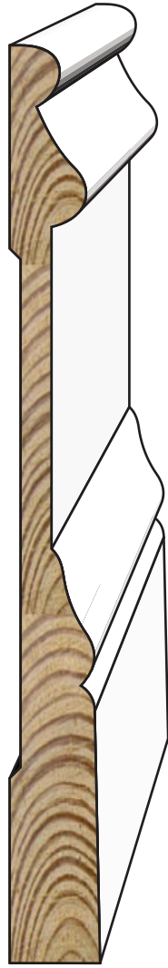
VB 9/16" x 5-1/4"
