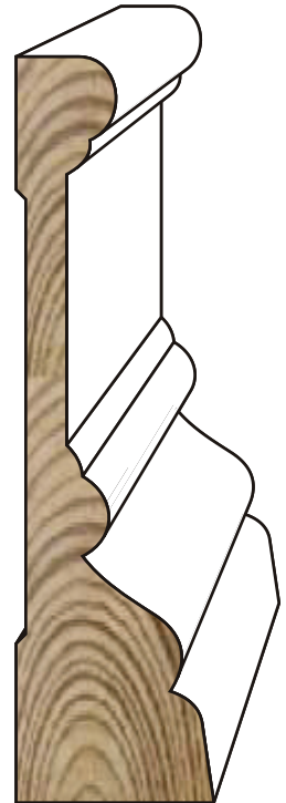
RB3 1" x 3-1/2"
